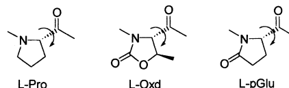
Figure 1. Chemical formula of L-Pro, L-Oxd, and L-pGlu; the rotatable bond is highlighted in each formula
